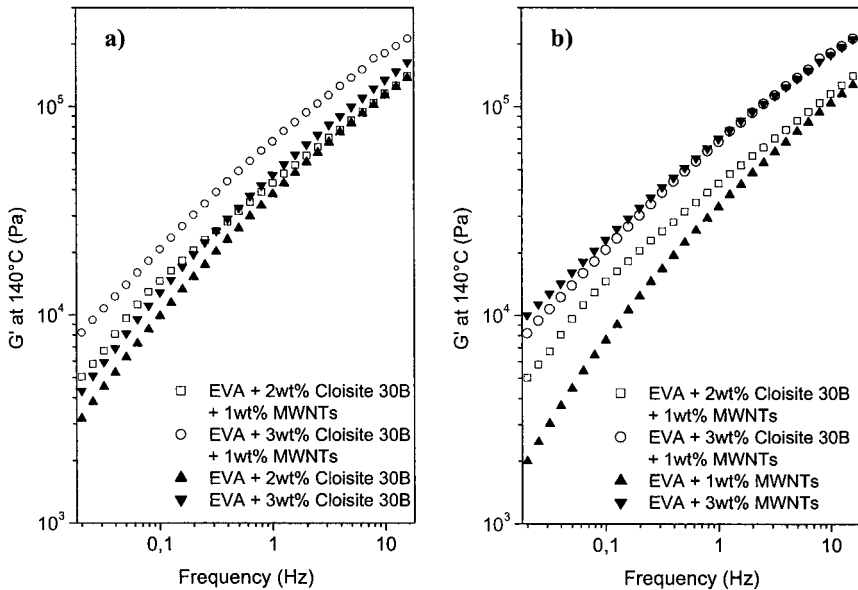
Figure 7. Frequency dependence of G' evolution at 140°C for binary and ternary systems a) comparison with EVA/organo clay binary compositions; b) comparison with EVA/MWNTs binary compositions.
