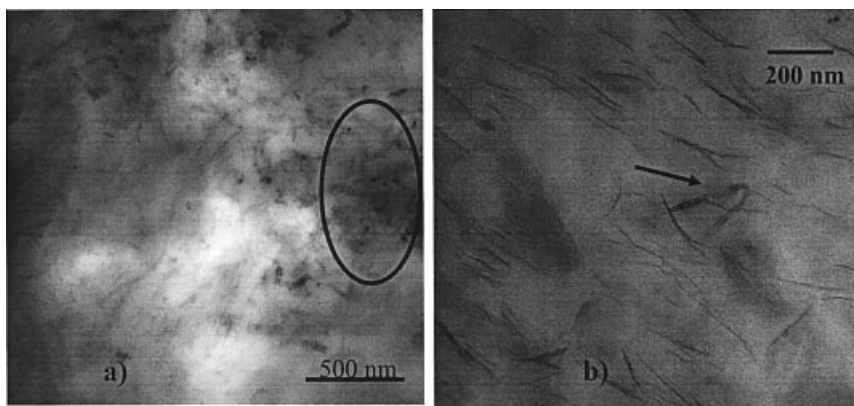
Figure 5. TEM micrographs of a ternary composite (3wt% Cloisite ® 30B+1wt% MWNTs). a) low magnification showing MWNTs aggregates b) high magnification showing stacks of clay and an isolated carbon nanotubes (a segment of which being highlighted by the arrow).
