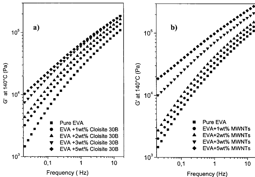
Figure 6. Frequency dependence of the storage modulus G' for binary nanocomposites at 140^{\circ}\text{C} : a) EVA + Cloisite ® 30B, b) EVA + MWNTs.
